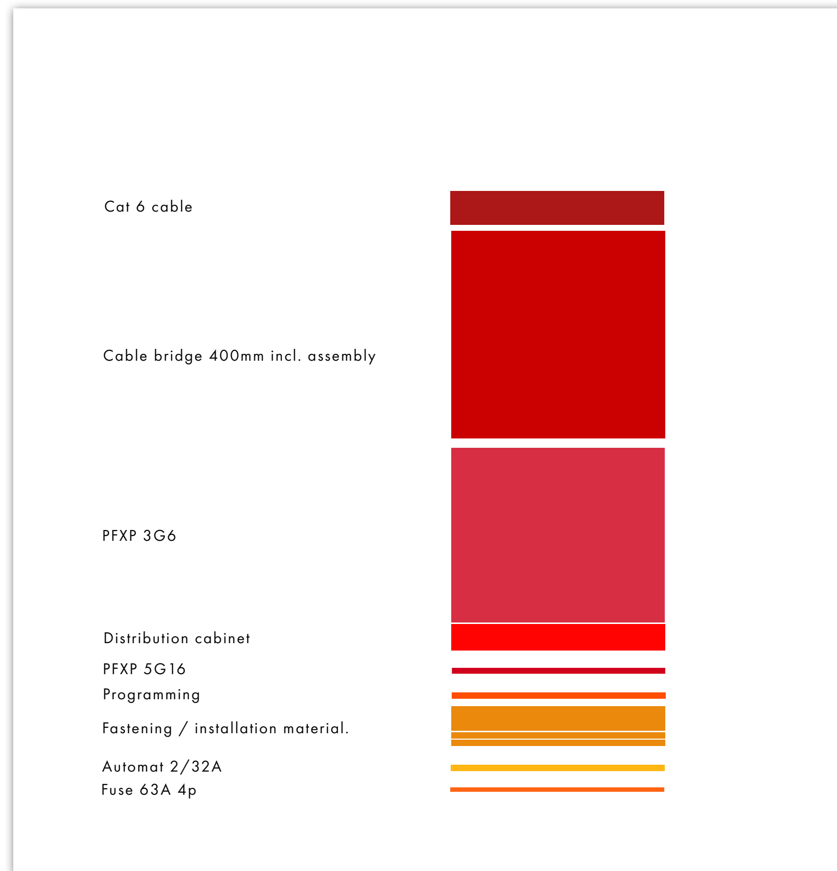
Traditional charging system
